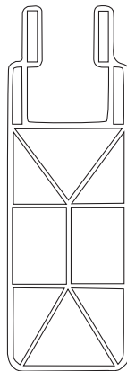
A02B 2" * 6" Enforcementfree Bottom Rail
